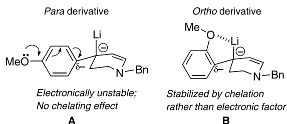
Figure 1. Possible stabilization of benzylic anion resulting from lithiation.
