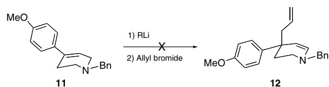
Scheme 2. Attempted allylation.
