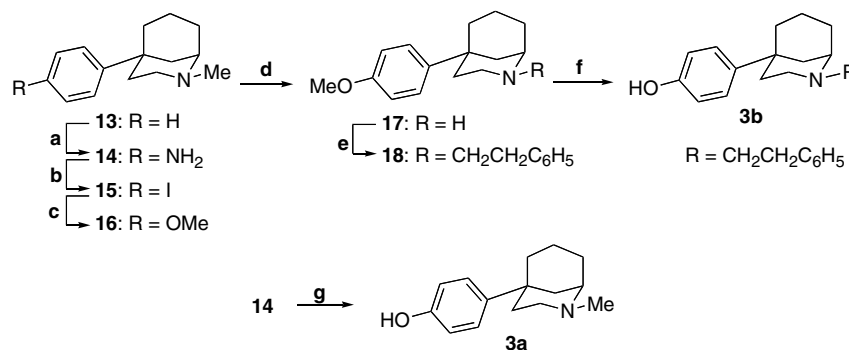
Scheme 3. Reagents and conditions: (a) i. 70% HNO 3 , 40 °C; ii. ethanol, 10% Pd-C, cat. AcOH, 60 °C, 83% over two steps; (b) concd HCl, NaNO 2 , then KI, 54%; (c) abs. MeOH, CuI (10 mol%), 1,10-phenanthroline (20 mol%), Cs 2 CO 3 , sealed tube, 80 °C, 89%; (d) i. abs. toluene, 2,2,2-trichloroethylformate, K 2 CO 3 , reflux; ii. 75% AcOH, Zn powder, rt, 61% over two steps; (e) i. CH 2 Cl 2 , phenylacetyl chloride, DMAP, 0 °C; ii. abs. THF, LiAlH 4 , 0 °C, 83% over two steps; (f) AcOH, 48% HBr, reflux, quantitative; (g) 35% H 2 SO 4 , NaNO 2 , H 2 O, urea, then Cu(NO 3 ) 2 , Cu 2 O, 58%.
