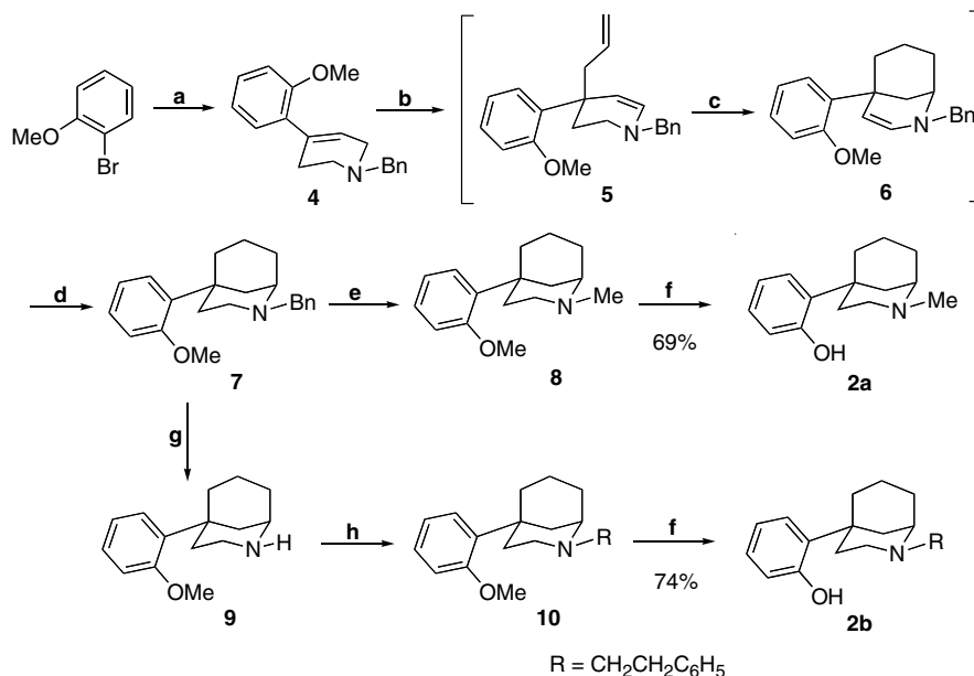
Scheme 1. Reagents and conditions: (a) i. THF, -78^{\circ}\text{C} , n\text{-BuLi} , then 1-benzyl-4-piperidone, to rt; ii. toluene, p\text{-toluenesulfonic acid monohydrate} , reflux, 71% over two steps; (b) THF, -50^{\circ}\text{C} , sec\text{-BuLi} , then allyl bromide, to 0^{\circ}\text{C} ; (c) \text{H}_3\text{PO}_4\text{--HCO}_2\text{H} (1:1), rt; (d) MeOH, 0^{\circ}\text{C} , \text{NaBH}_4 , then rt, 66% over three steps; (e) MeOH, 10% Pd-C, 37% \text{HCHO} in \text{H}_2\text{O} , cat. AcOH, \text{H}_2 , 60^{\circ}\text{C} , 85%; (f) AcOH, 48% \text{HBr} , reflux; (g) MeOH, 10% Pd-C, cat. AcOH, 60^{\circ}\text{C} , 92%; (h) (i) \text{CH}_2\text{Cl}_2 , phenylacetyl chloride, DMAP, 0^{\circ}\text{C} ; (ii) THF, \text{LiAlH}_4 , 0^{\circ}\text{C} , 92% over two steps.
